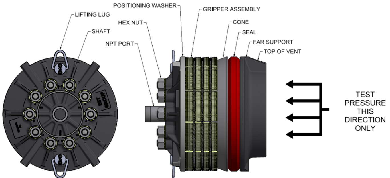
GripTight MAX High Pressure Test Plug
